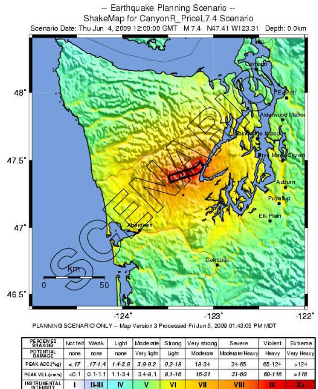
Figure 1. ShakeMap for a M7.4 earthquake on the Canyon River–Saddle Mountain fault zone. The black polygon is the modeled fault rupture surface.
